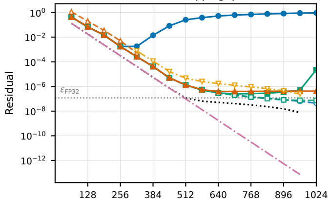
(a) Residual and stopping quantities
