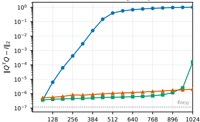
(b) Loss of orthogonality
