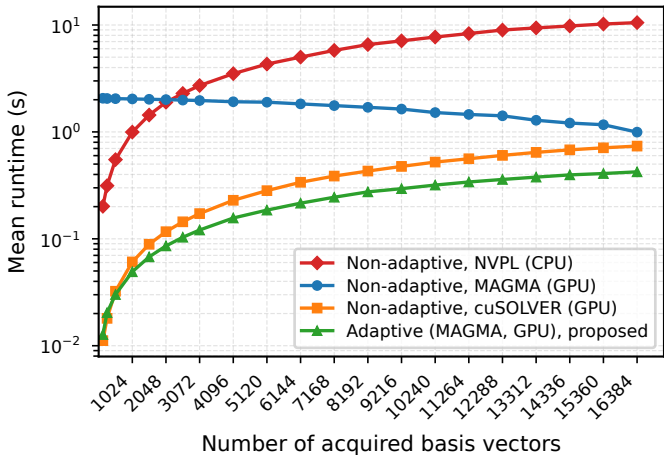
Householder range finder runtime, M = N = 16\,384
