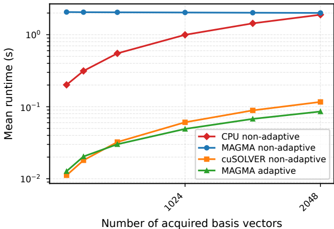
Rangefinder runtime, M = N = 16384
