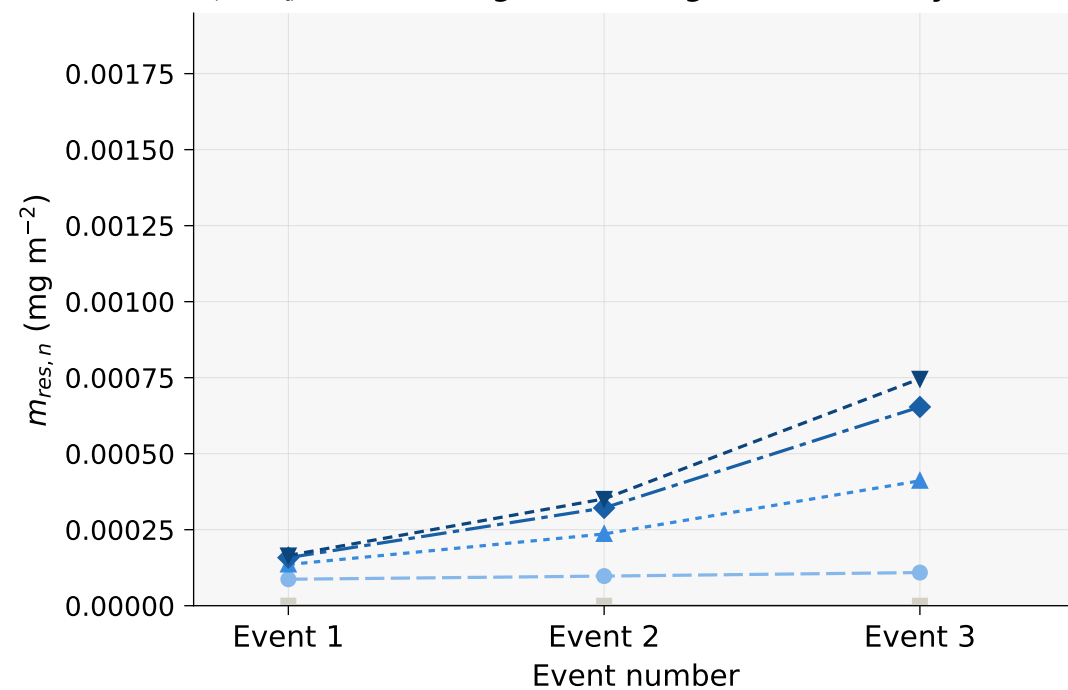
Freundlich isotherm — single application K_f = K_d, N=0.85 \cdot \text{dgPin} = 1.0 \text{ mg/m}^2 \text{ event 1 only}
