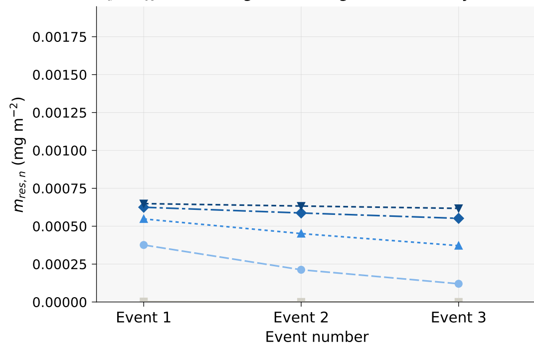
Linear isotherm — single application K_d = K_{oc} \times \text{OC}\% \cdot \text{dgPin} = 1.0 \text{ mg/m}^2 \text{ event 1 only}
