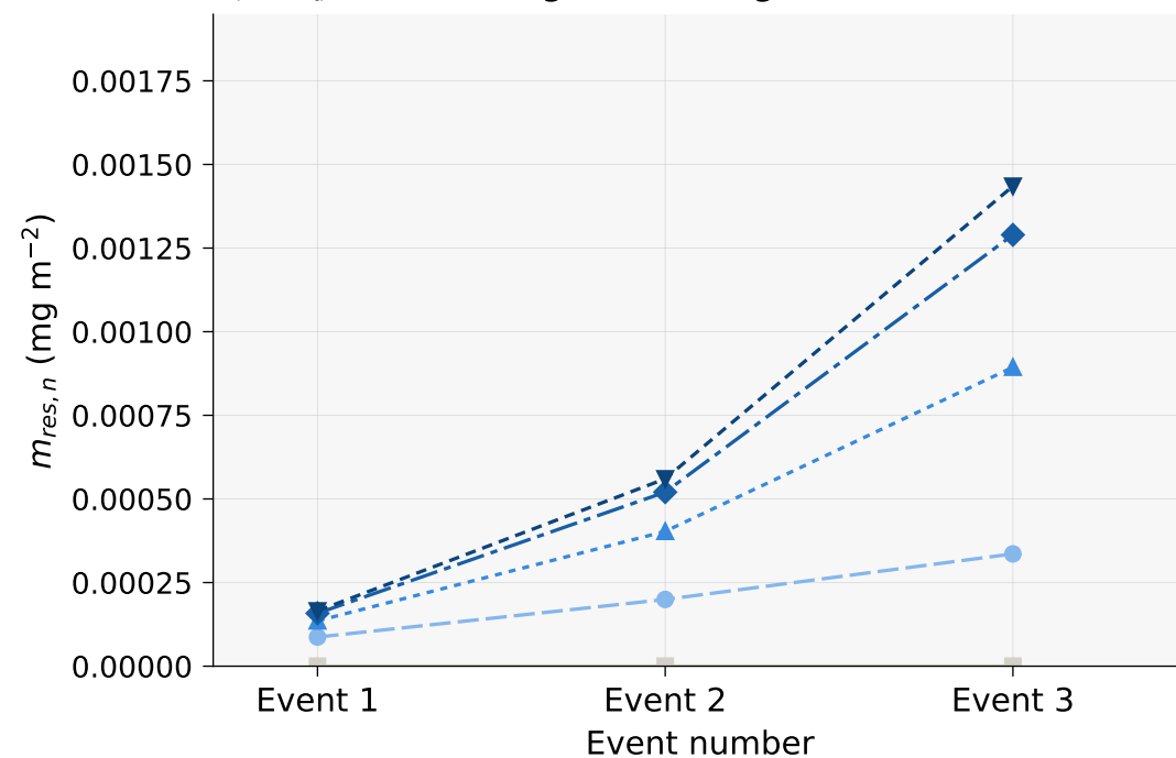
Freundlich isotherm — all events K_f = K_d, N=0.85 \cdot \text{dgPin} = 1.0 \text{ mg/m}^2 \text{ each event}
