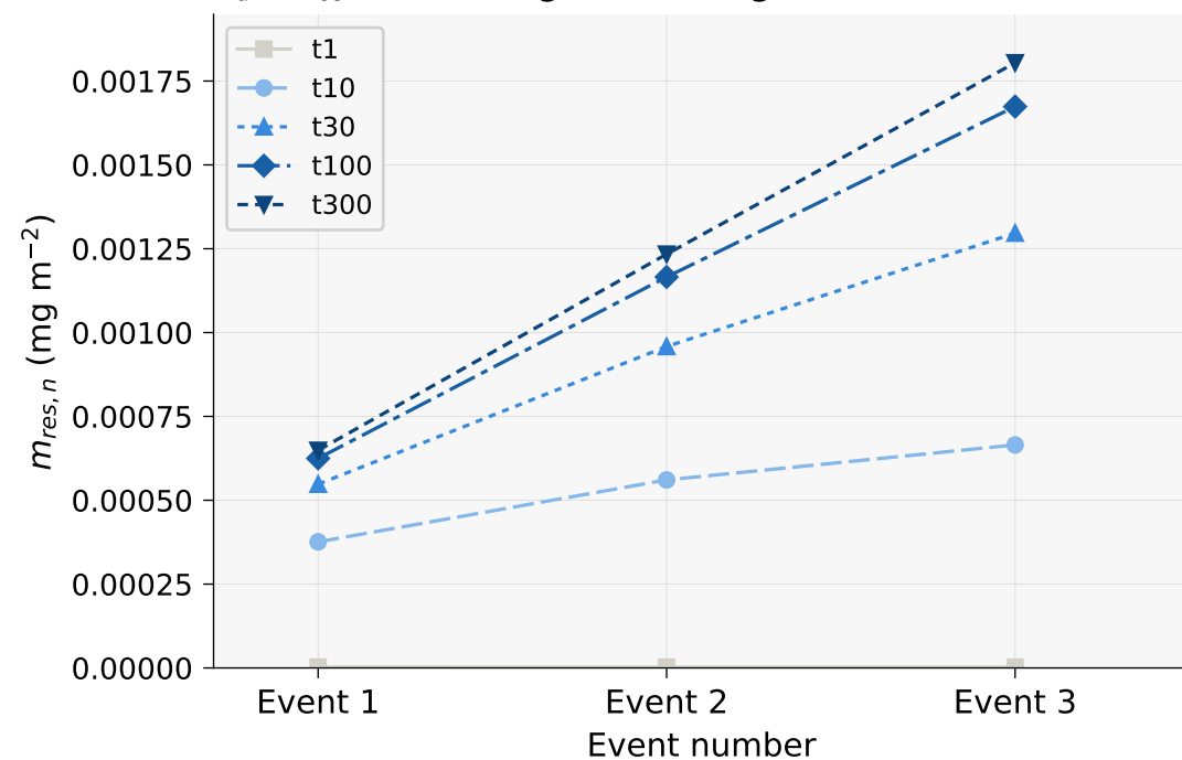
Linear isotherm — all events K_d = K_{oc} \times \text{OC}\% \cdot \text{dgPin} = 1.0 \text{ mg/m}^2 \text{ each event}
