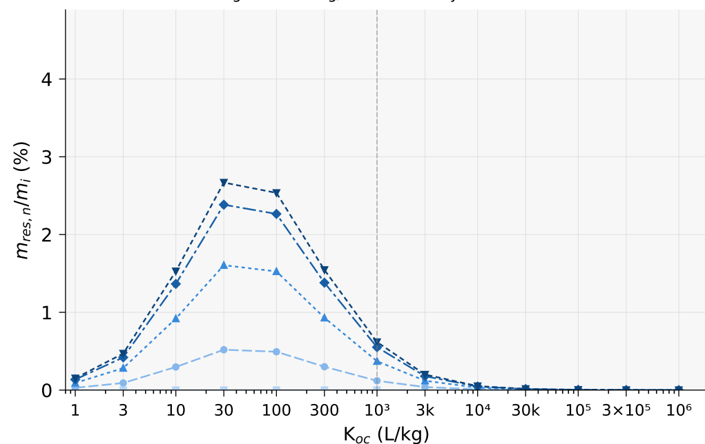
c) Linear — single application K_d = K_{oc} \times 1\%OC · dgPin = 0.1 mg/m 2 event 1 only
