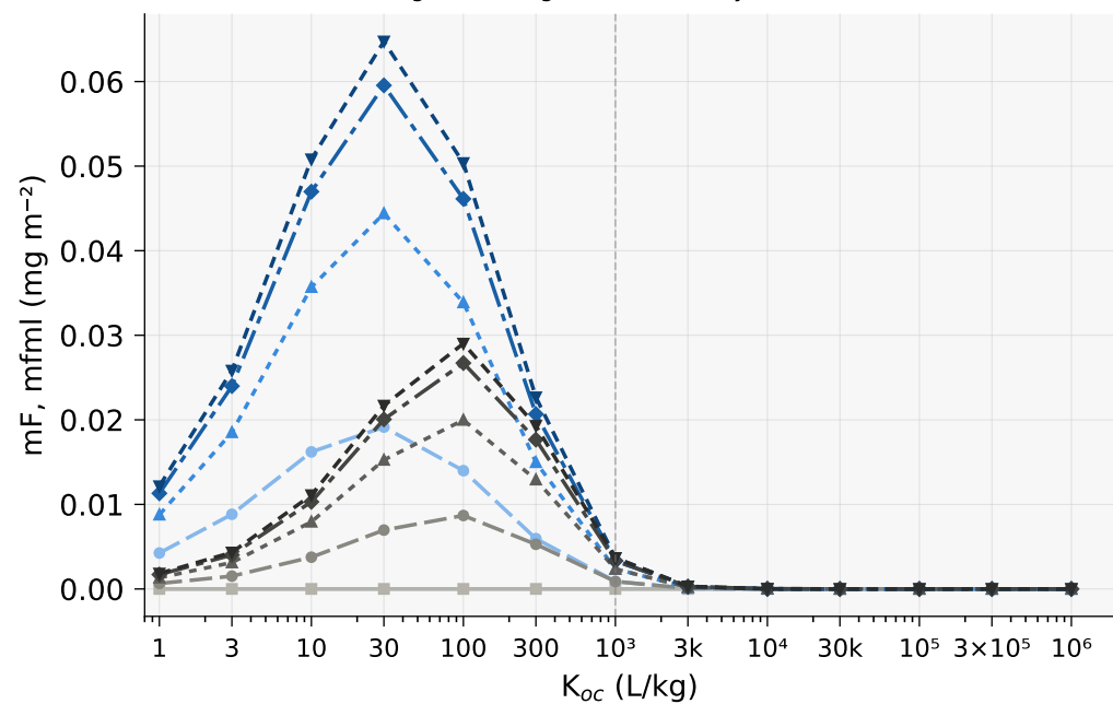
d) Freundlich — single application K_f = K_d \cdot N=0.85 · dgPin = 1 mg/m 2 event 1 only
