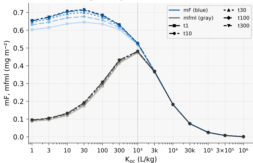
a) Linear — all events K_d = K_{oc} \times 1\%OC · dgPin = 1 mg/m 2 each event
