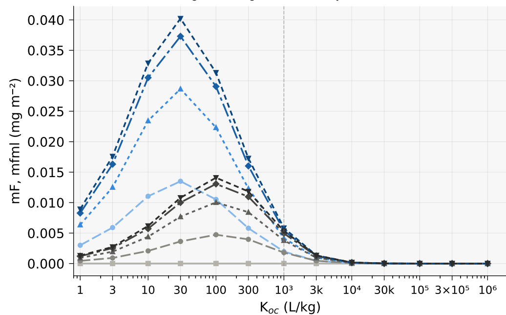
c) Linear — single application K_d = K_{oc} \times 1\%OC · dgPin = 1 mg/m 2 event 1 only
