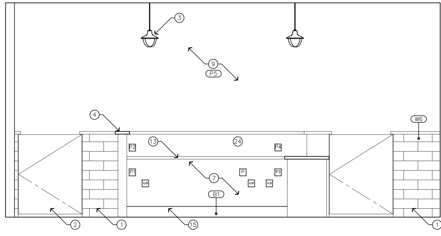
D ELEVATION
