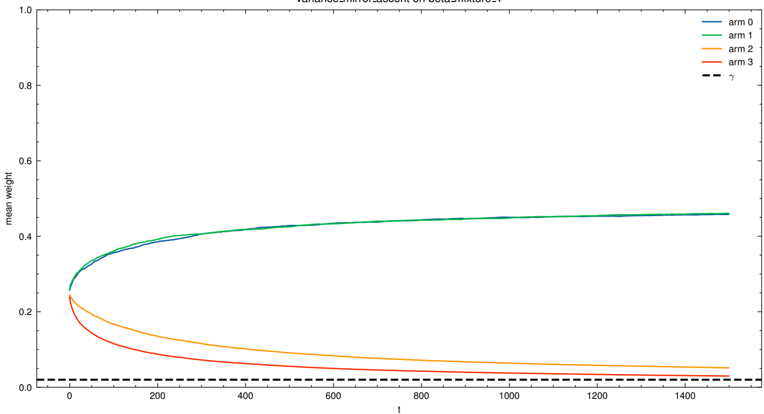
variance_if_ascent on beta_mixture_4
