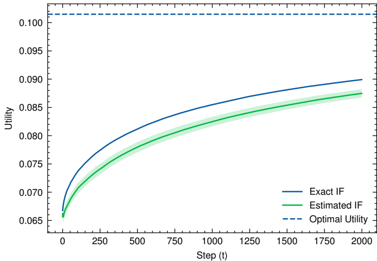
Variance Utility on beta_mixture_4
