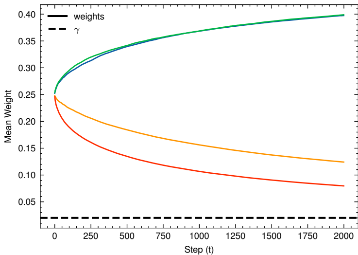
Estimated IF on beta_mixture_4
