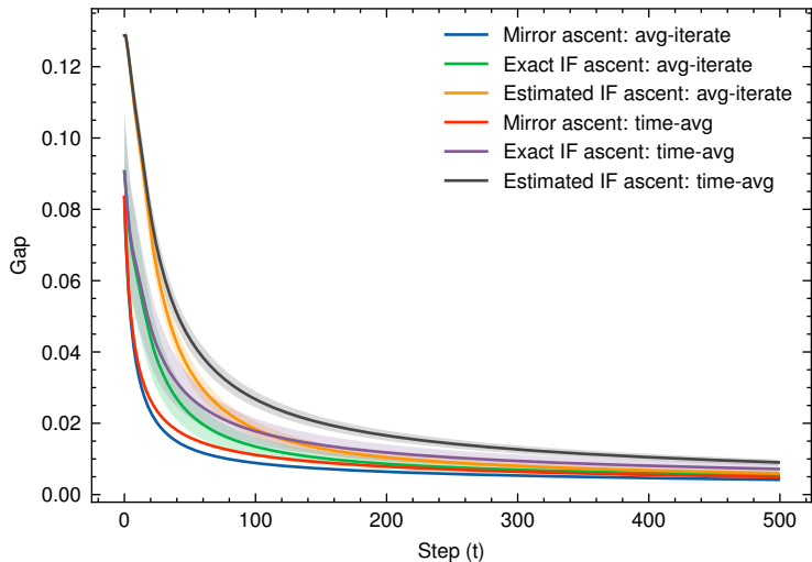
Avg-Weight Gap and Time-Averaged Gap on beta_mixture_4
