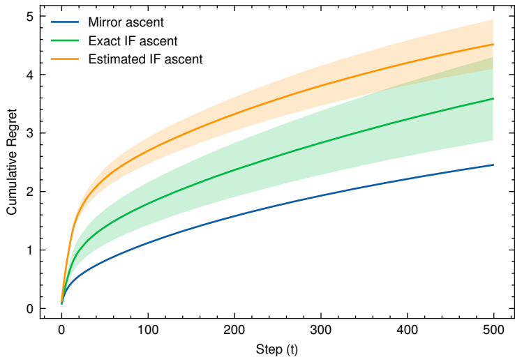
Cumulative Regret on beta_mixture_4
