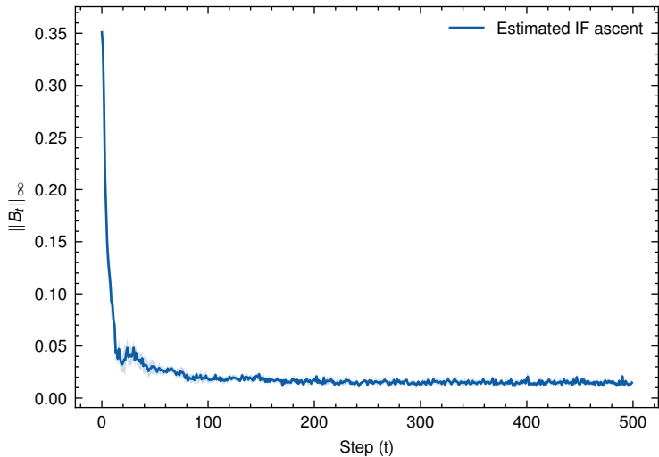
Monte Carlo Bias Norm on beta_mixture_4
