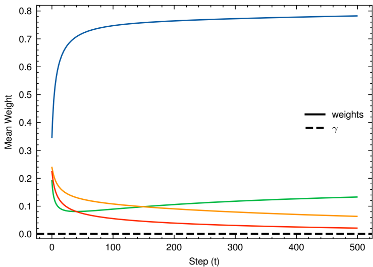
Exact IF ascent on beta_mixture_4
