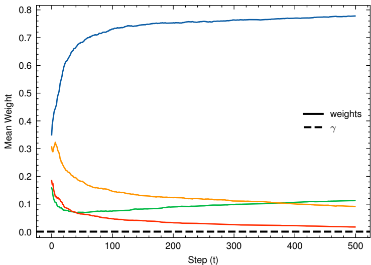
Estimated IF ascent on beta_mixture_4
