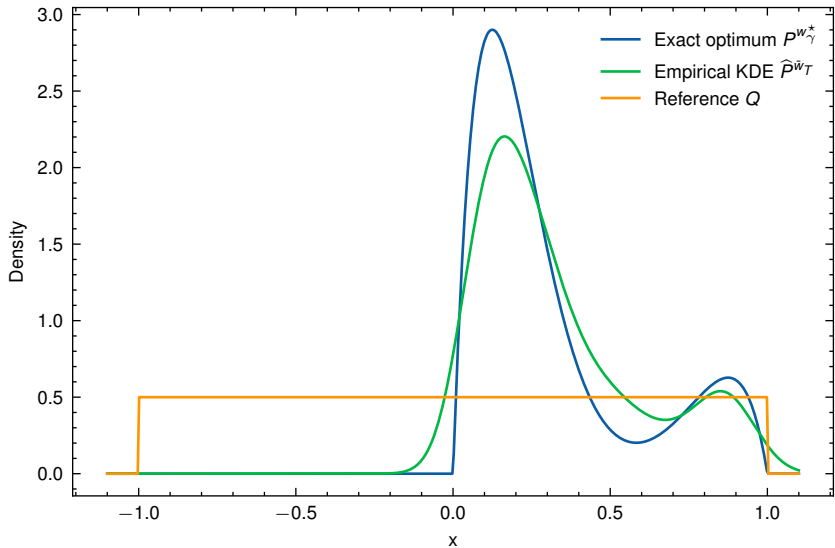
beta_mixture_4 - seed 100
