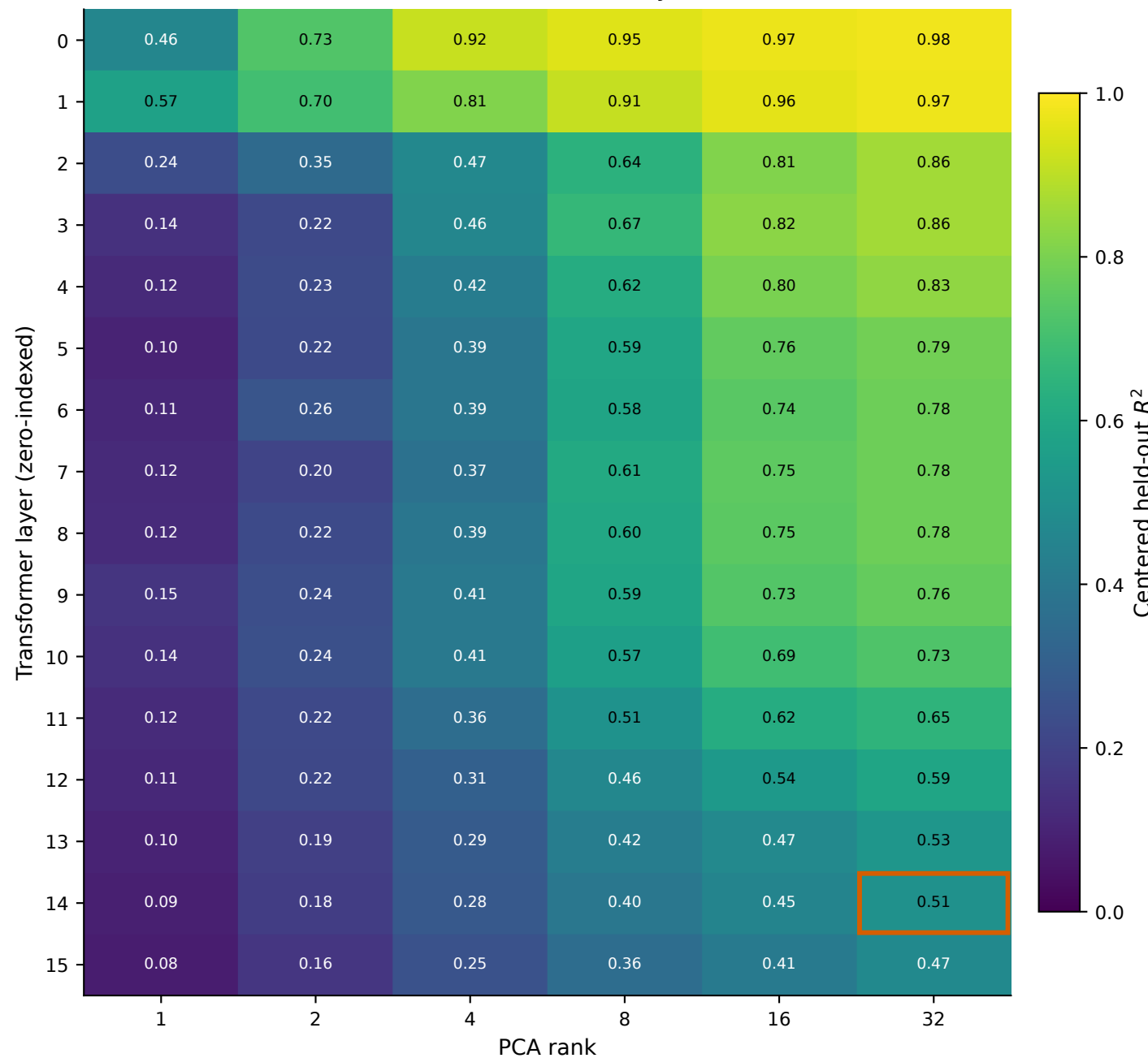
Held-out reconstruction across layers and ranks
