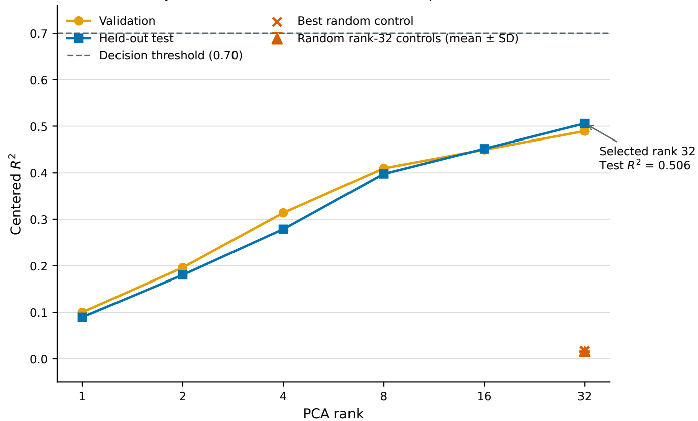
Layer 14 rank curve and random-subspace control
