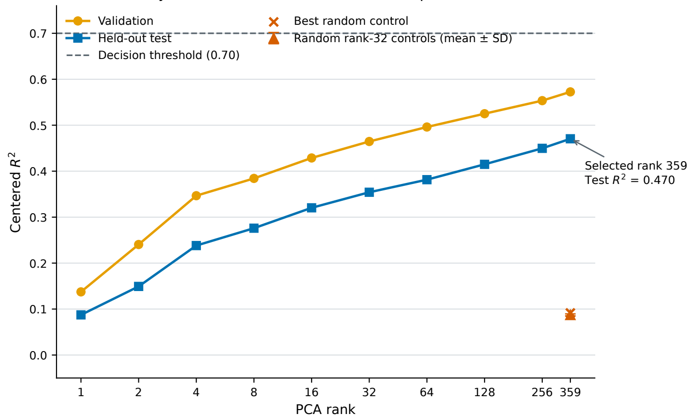
Layer 28 rank curve and random-subspace control
