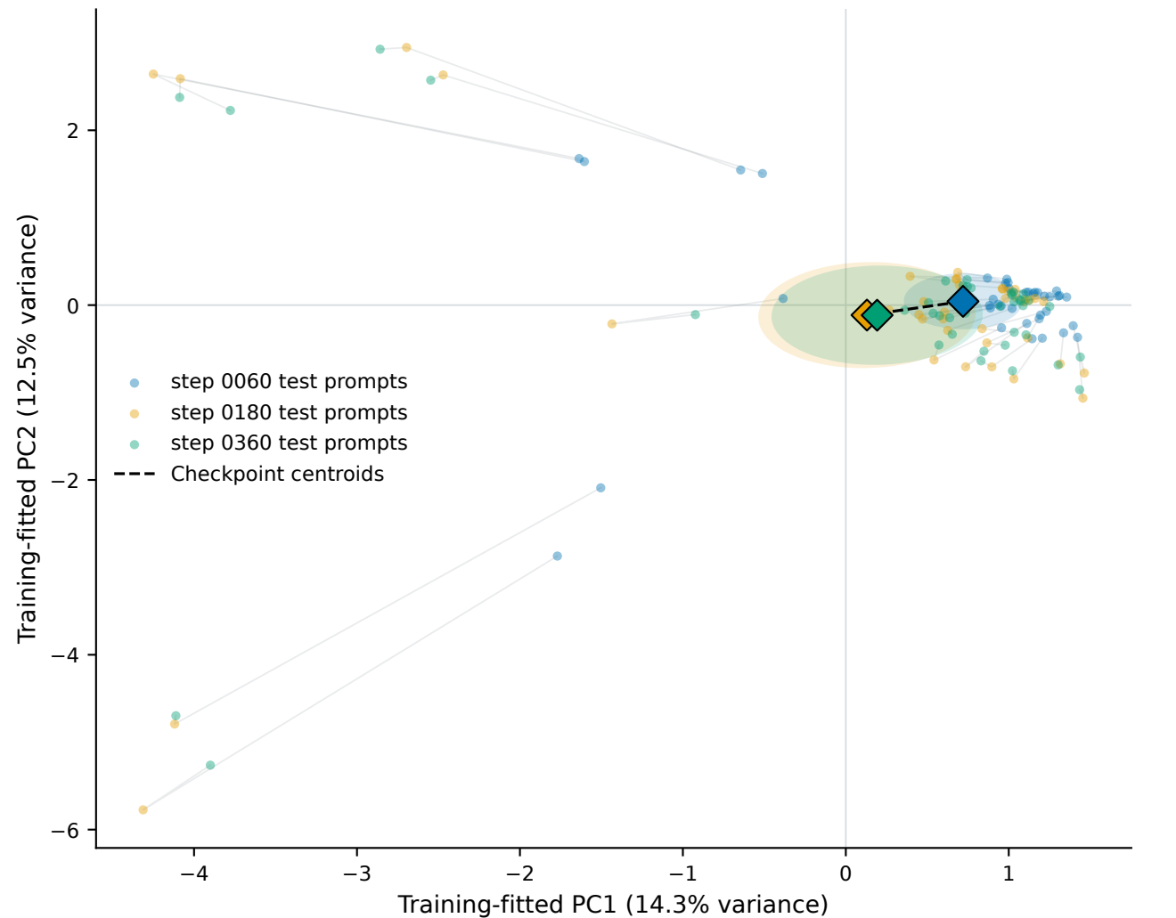
Held-out prompt trajectories in a training-fitted 2D projection
