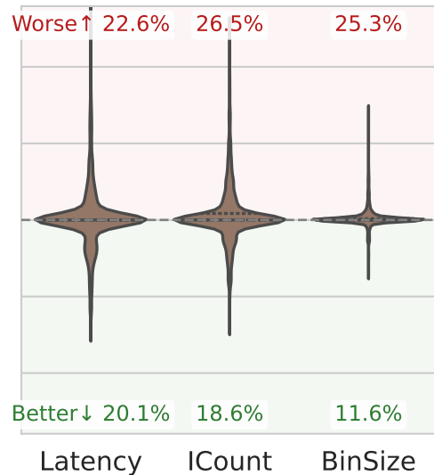
Model_Latency_3B vs instcombine
