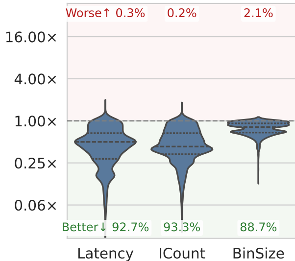
instcombine vs -O0
