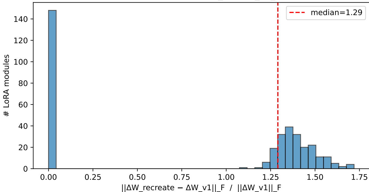
Per-layer LoRA delta divergence (lora_v1 vs L_v1_recreate, n=353)
