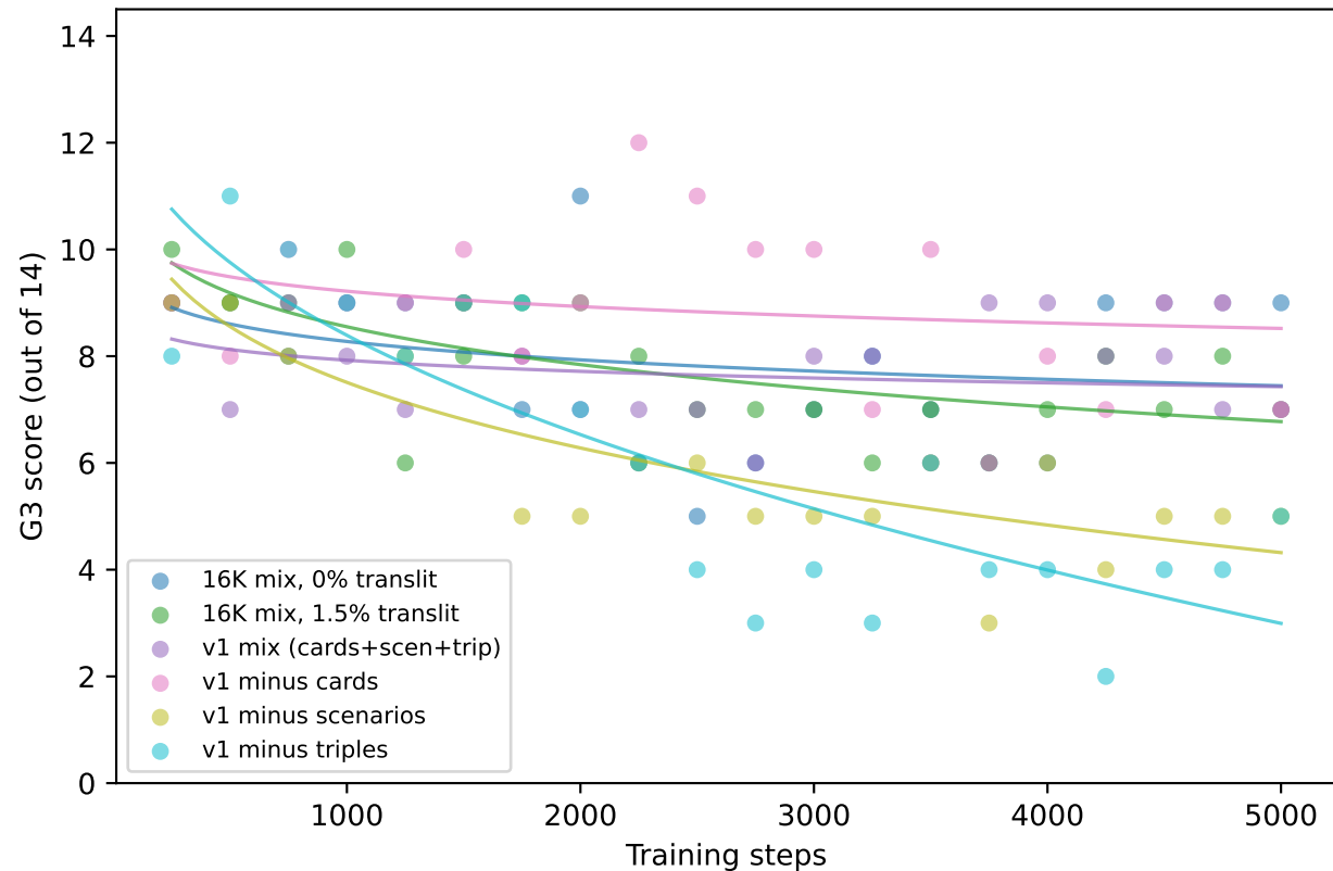
Forgetting power-law: G3 (JSON parse) vs train step
