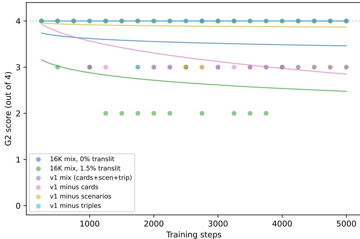
Forgetting power-law: G2 (transliteration) vs train step
