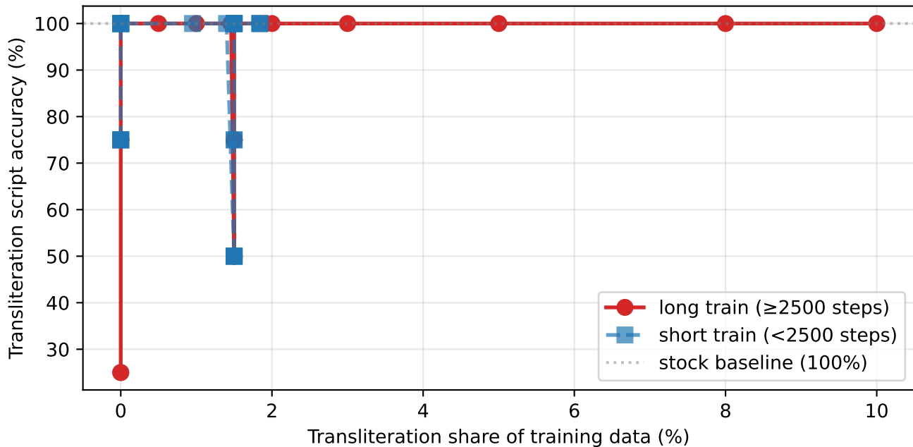
Policy-Frequency \times Training-Duration Interaction (E2B base, transliteration policy)
