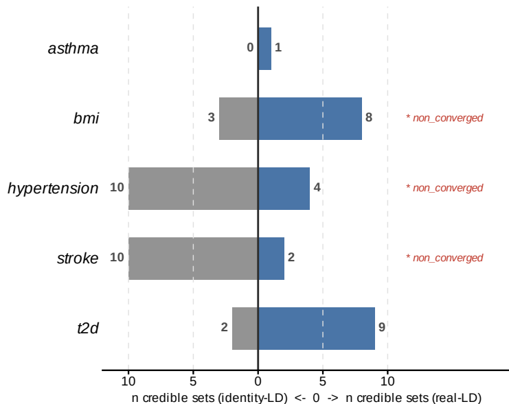
Figure 3. Structural collapse of identity-LD signal at SH2B3 12q24 EUR under real-LD re-analysis.
