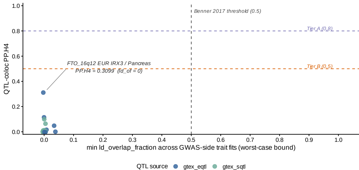
Figure H3. LD-reference-quality dose-response on coloc inference at admissible TrackA loci.
