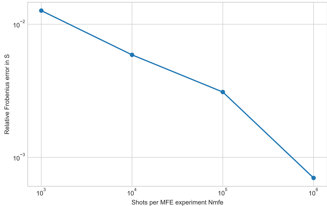
standard overlap error vs finite MFE shots
