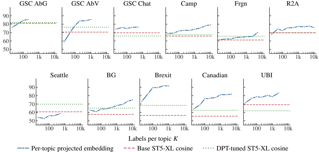
Test accuracy (%)
