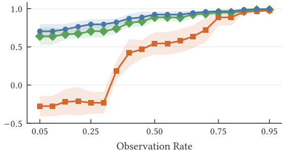
Kendall's \tau under Pol.is Routing
