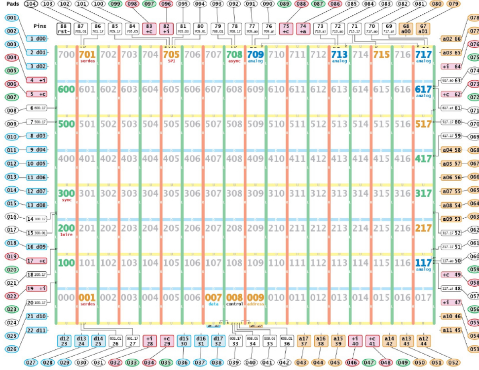
Figure 1: GA144A12 array layout and pin designation, showing the 18 by 8 node fabric, communication-port directions, I/O-capable nodes, boot specializations, analog nodes, and external pin mapping. Adapted from the GA144A12 revision A12 datasheet [7].
