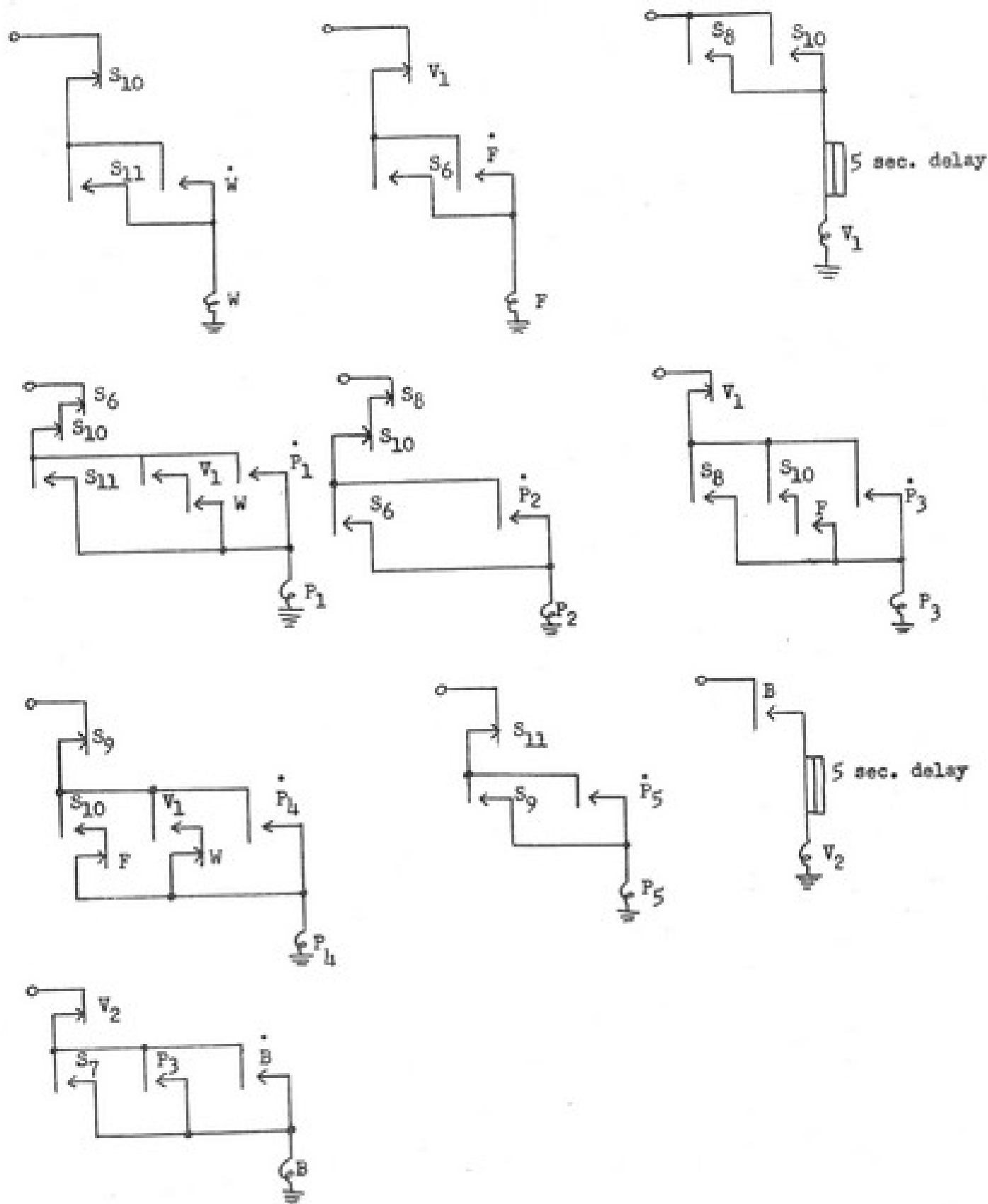
Figure 10 -- Robot Life Species No. 1 -- Programming Circuits
