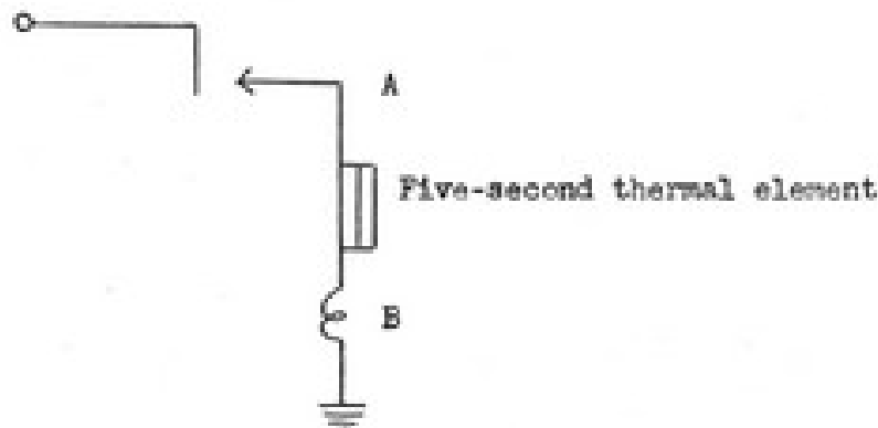
Figure 8 -- A Five-Second Delay Function
