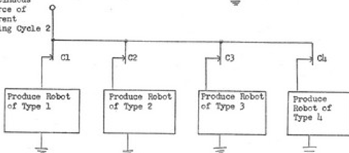
Figure 4 -- Schematic for the Birth Factory
