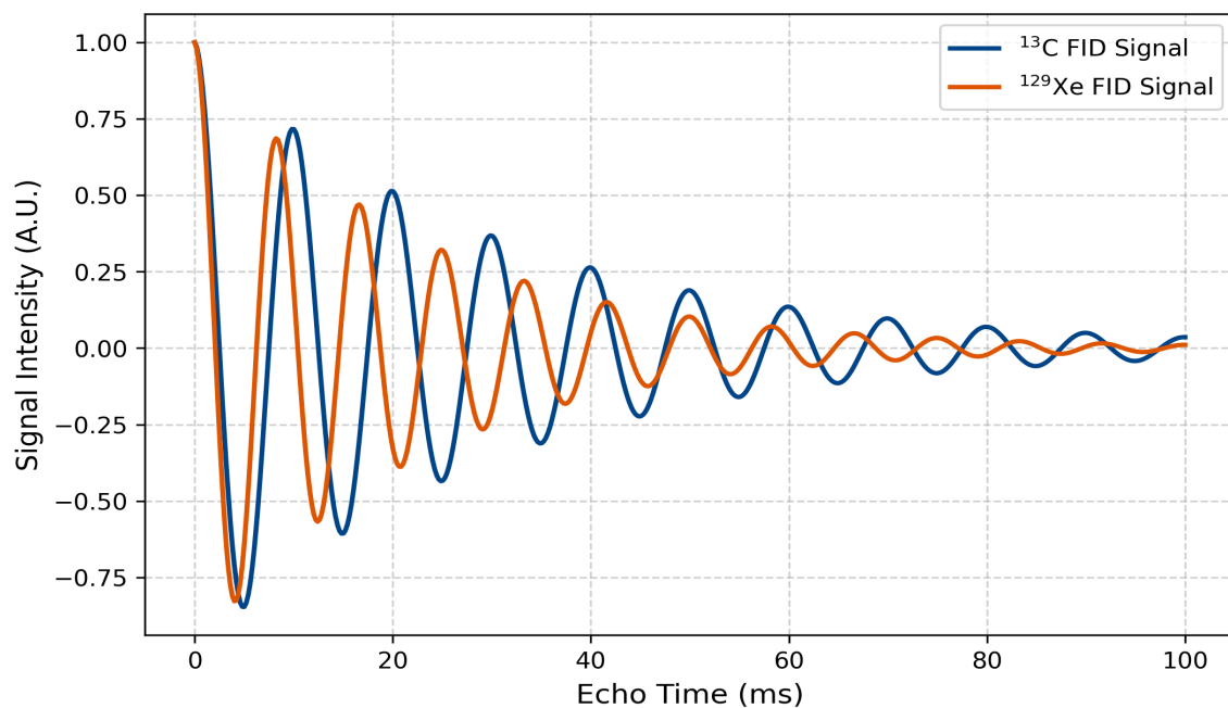
Free Induction Decay & Thermal Progression
