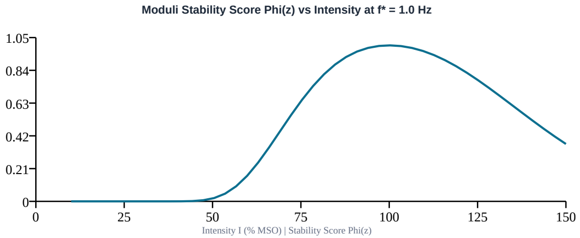
Figure 1 | Moduli stability function \Phi(z) along the optimal frequency cross-section, showing resonance peaks corresponding to fundamental domain elliptic boundaries.
