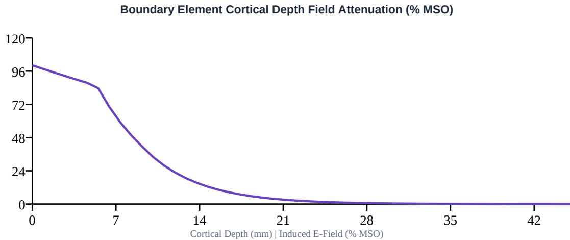
Figure 2 | Boundary element electric field attenuation across concentric tissue layers (scalp, skull, CSF, grey matter) computed from the moduli-optimal protocol.
