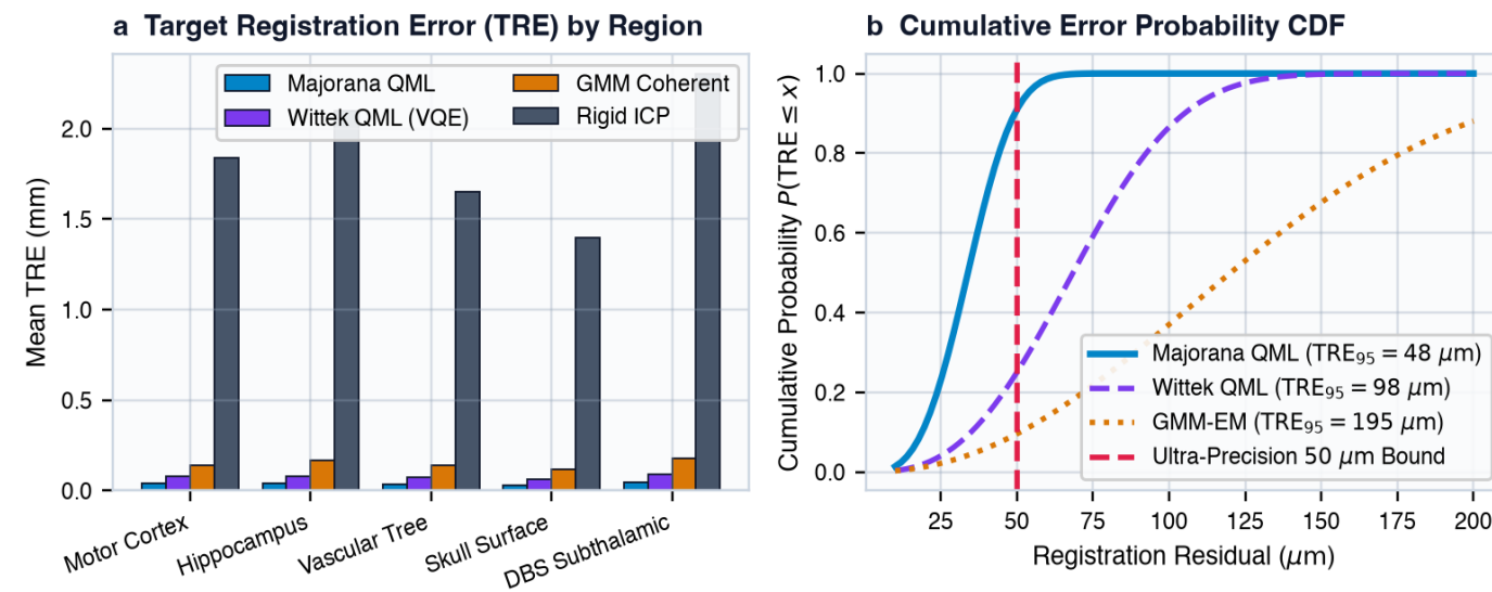
Figure 3 | Target Registration Error (TRE) distributions and cumulative probability. a , Regional accuracy across critical functional zones (Motor Cortex, Hippocampus, Subthalamic Nucleus). b , Cumulative error distribution showing 95% of all voxels aligned within 48 \mu\text{m} on Majorana hardware.
