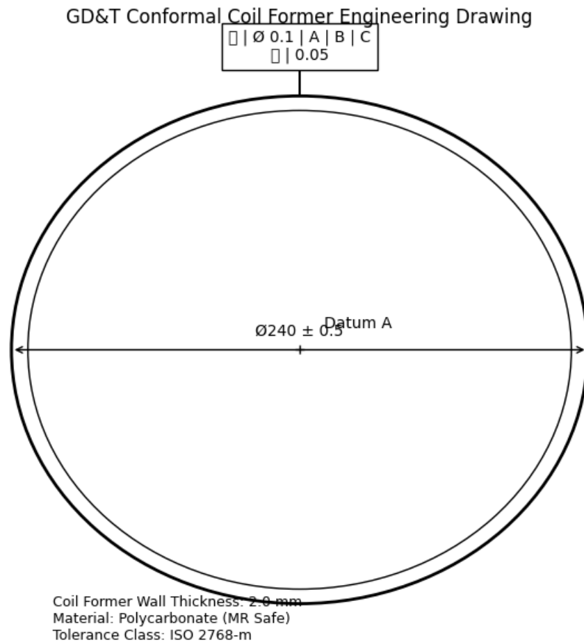
Figure 1: GD&T; Engineering Drawing for the coil former showing True Position and Cylindricity tolerances critical for maintaining conformality.
