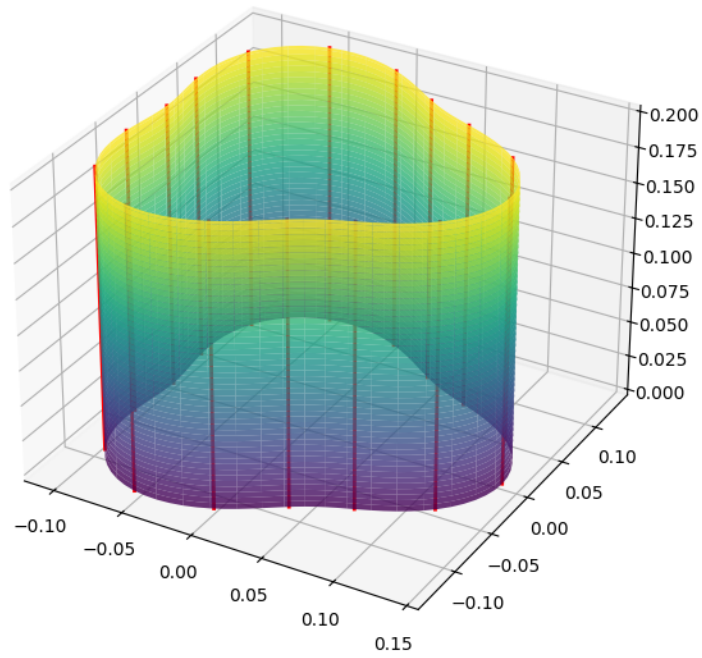
Figure 2: 3D geometry layout of the conformal coil array elements.
