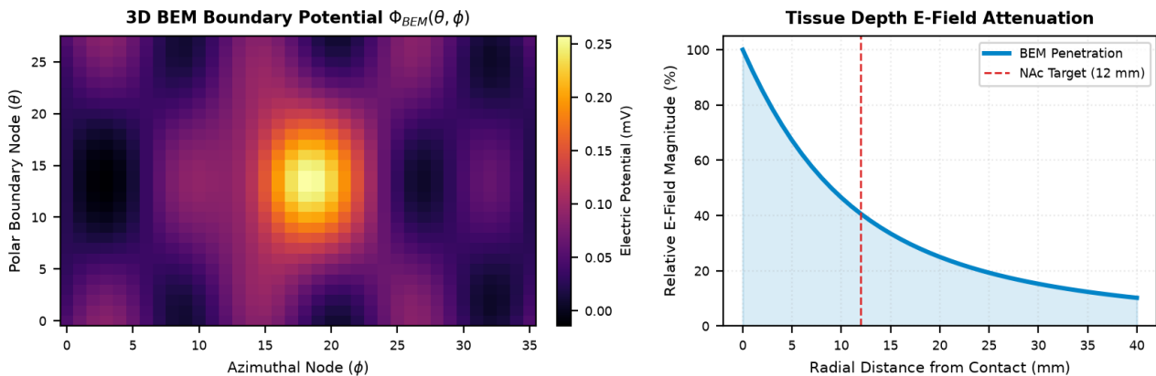
Figure 1 | Boundary Element Method (BEM) Field Simulation. Left: 3D boundary potential map \Phi_{BEM}(\theta, \phi) exhibiting high dipolar localization at the subcortical target interface. Right: Radial tissue depth electric field attenuation demonstrating critical 12 mm therapeutic field maintenance within safe charge injection limits.
