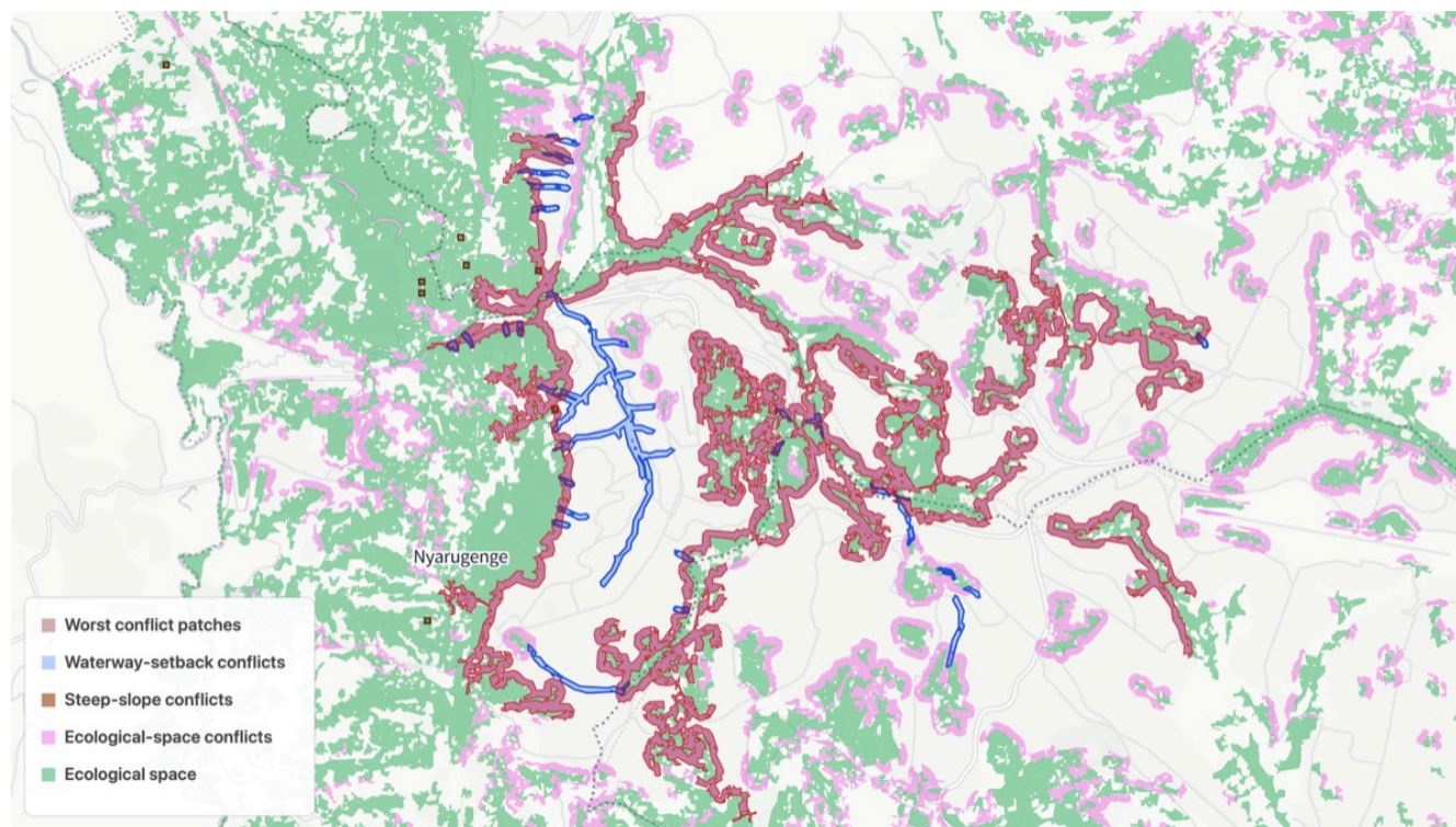
The Kigali run as delivered: ecological space with the three conflict families and the worst-patch ranking
