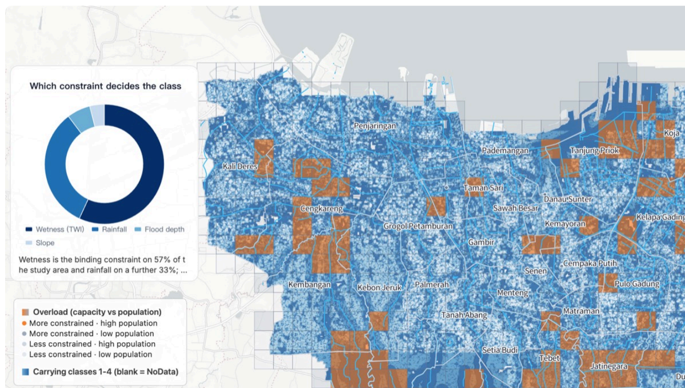
The Jakarta scenario as delivered: carrying-capacity classes 1–4, overload cells and the constraint-composition chart
