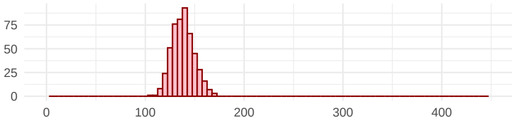
Bootstrap distribution of sample means
