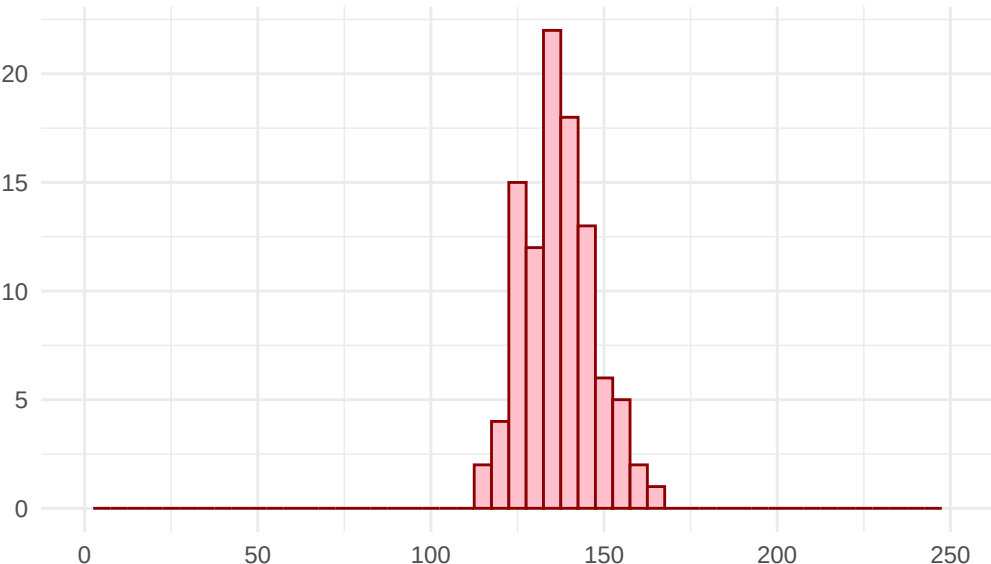
Bootstrap distribution of sample means
