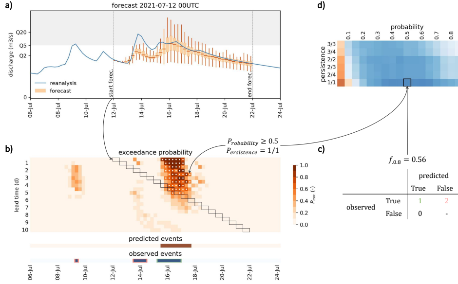
Figure 1: Overview of the skill assessment framework. a) Hydrographs comparing observed and forecasted discharge with the discharge associated to the 5-year return period. b) Matrix of total exceedance probability (white dots identify pairs of date and lead time that meet the notification criteria, whereas black rectangles delineate the location of the forecast hydrograph from panel (a) in the probability matrix) and identification of predicted events for specific values of probability threshold and persistence. c) Confusion matrix for the selected station, constructed based on the previous notification criteria. d) Evaluation of the f-score across all combinations of probability threshold and persistence; the black square highlights the skill score corresponding to the notification criteria in panel (b).
