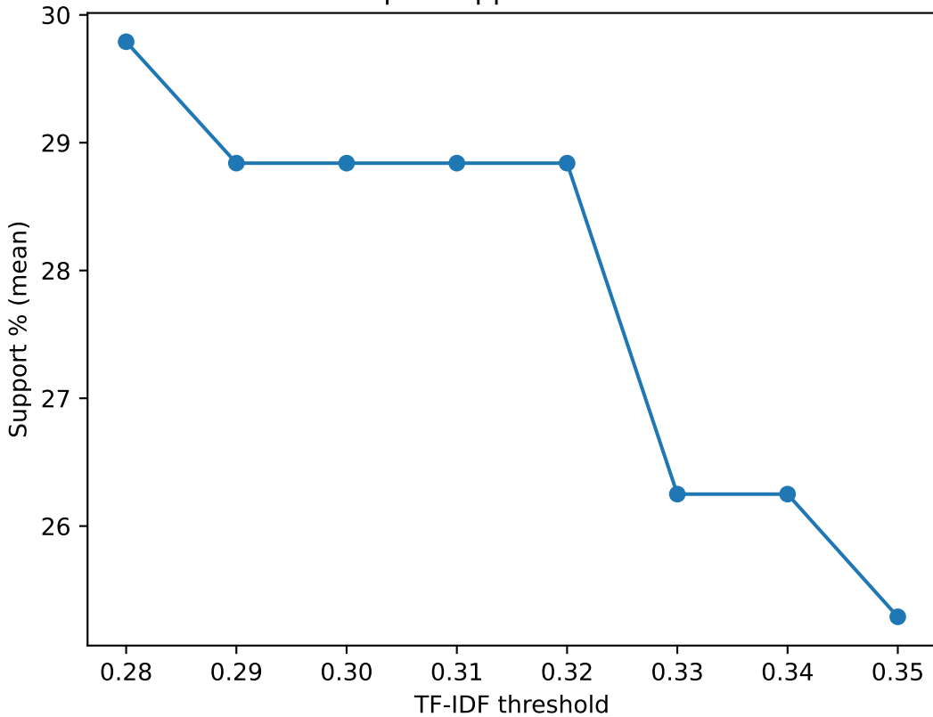
Graph: Support vs TF-IDF
