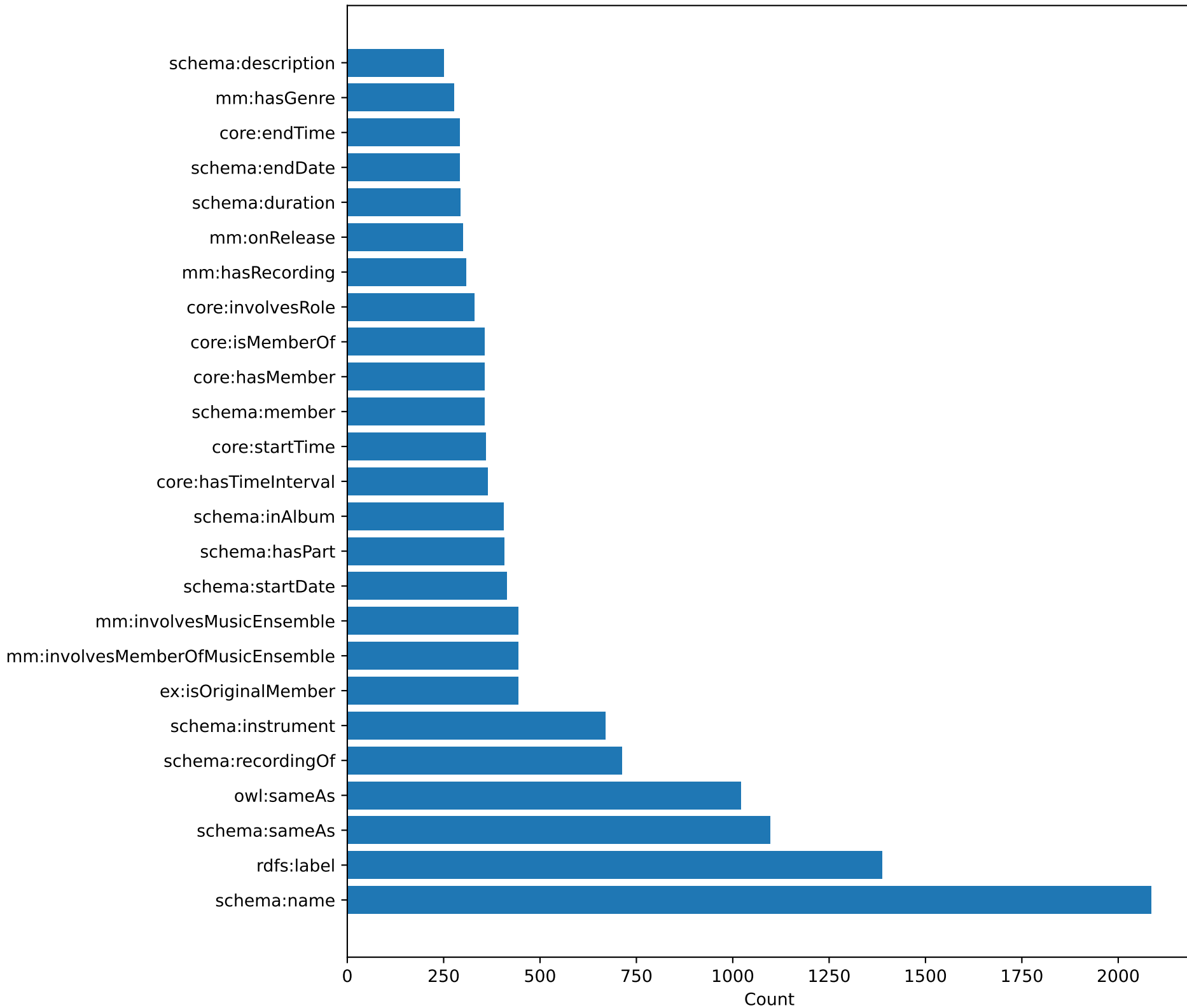
Top predicates (excluding rdf:type)
