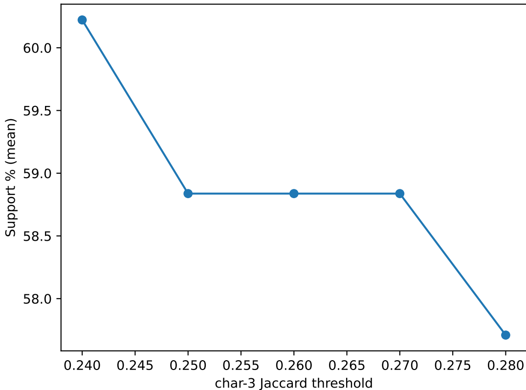
Hybrid: Support vs char-3
