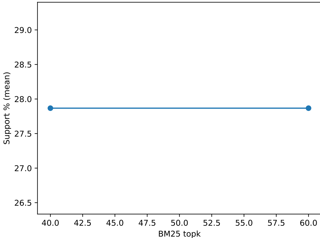
Graph: Support vs BM25 topk (filter)
