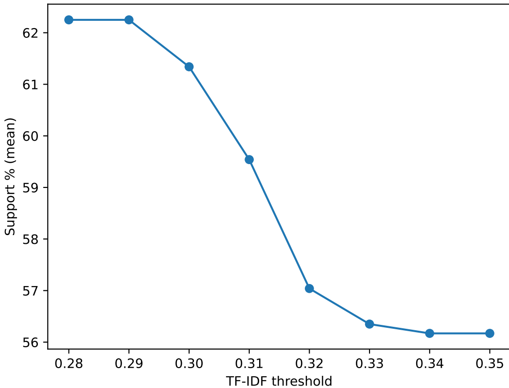
Hybrid: Support vs TF-IDF
