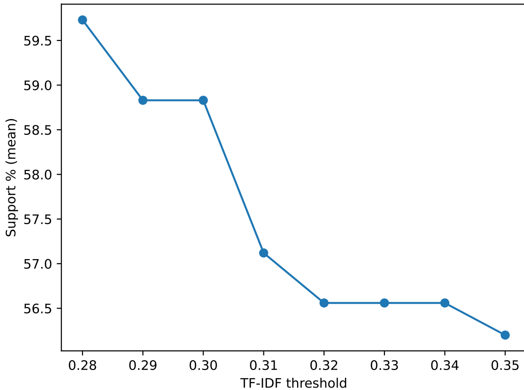
KG: Support vs TF-IDF
