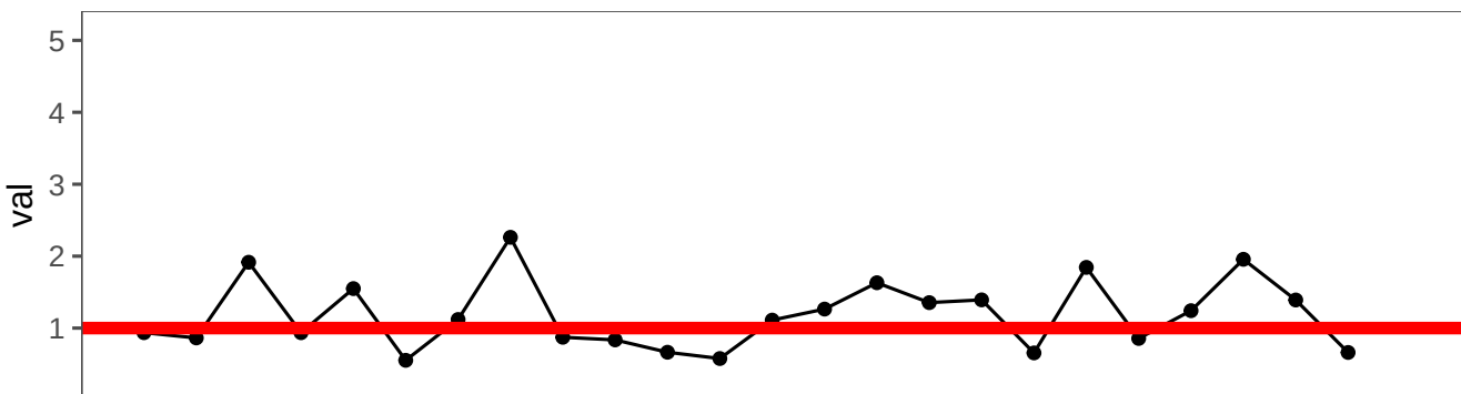
evaporative_index
