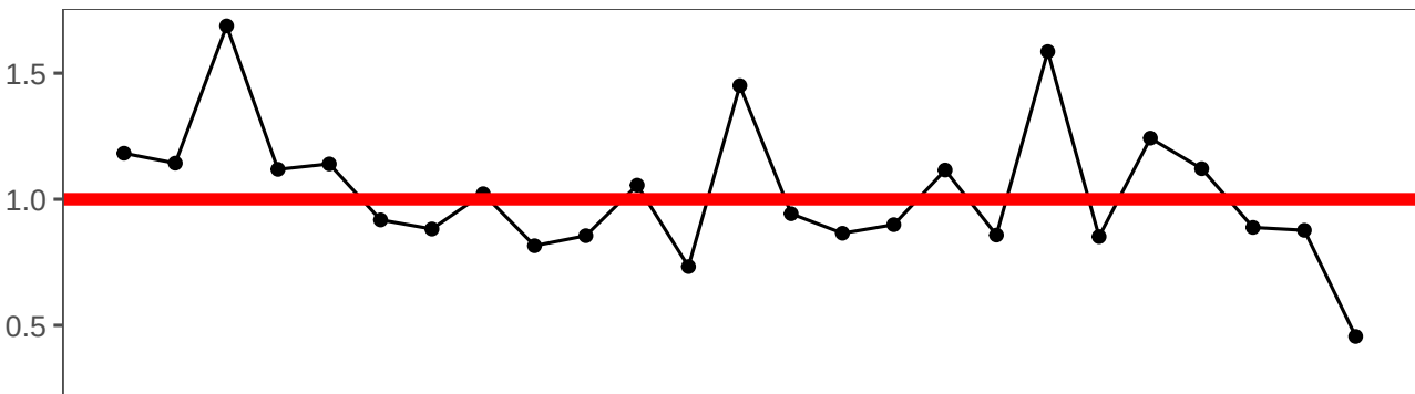
evaporative_index
