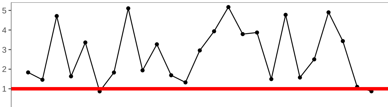
aridity_index
