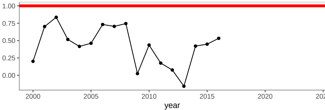
ratio
