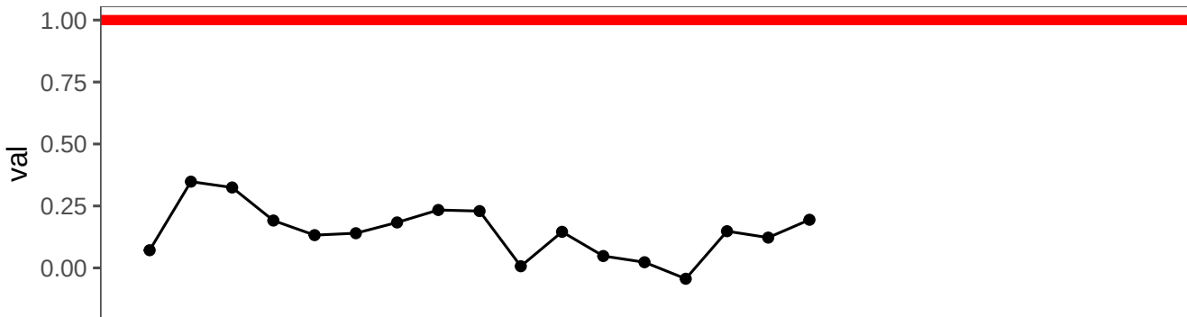
ei_obs
