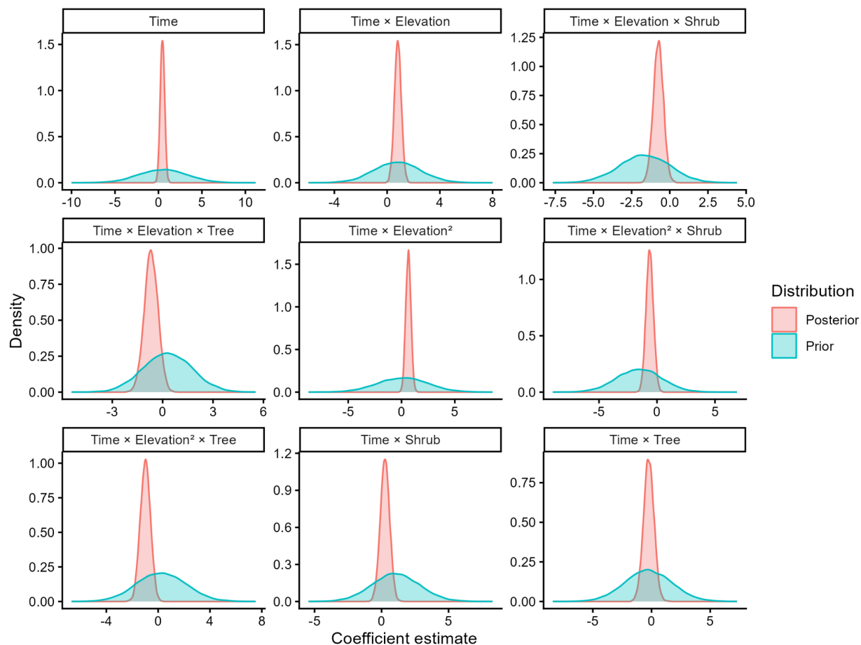
Figure S10.C. Prior (blue) and posterior (red) distributions for fixed-effect coefficients in the Bayesian model. Coefficients include time, time \times elevation, time \times elevation 2 , and interactions between time and functional group (shrub and tree), including their interactions with elevation and elevation 2 .
