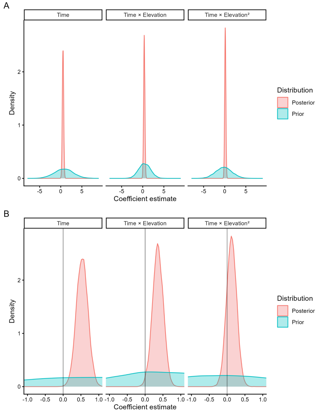
Figure S6.A. Prior (blue) and posterior (red) distributions for key fixed-effect coefficients in the Bayesian model. (A) Relocation-error-informed prior and posterior distributions for the effects of time, time \times elevation, and time \times elevation 2 . (B) Same distributions shown on a narrower coefficient scale (-1 to 1) to highlight the posterior distributions in proximity to 0.
