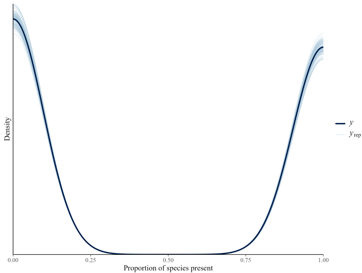
Figure S6.B. Posterior predictive check of the full model with informative priors. The consistency of the real data and simulated data demonstrate that the model accurately characterizes the data in this density graph. The simulated data is shown by the dark blue curve ( y ) and observed data is shown by the light blue curves ( y_{\text{rep}} , n = 100 ).
