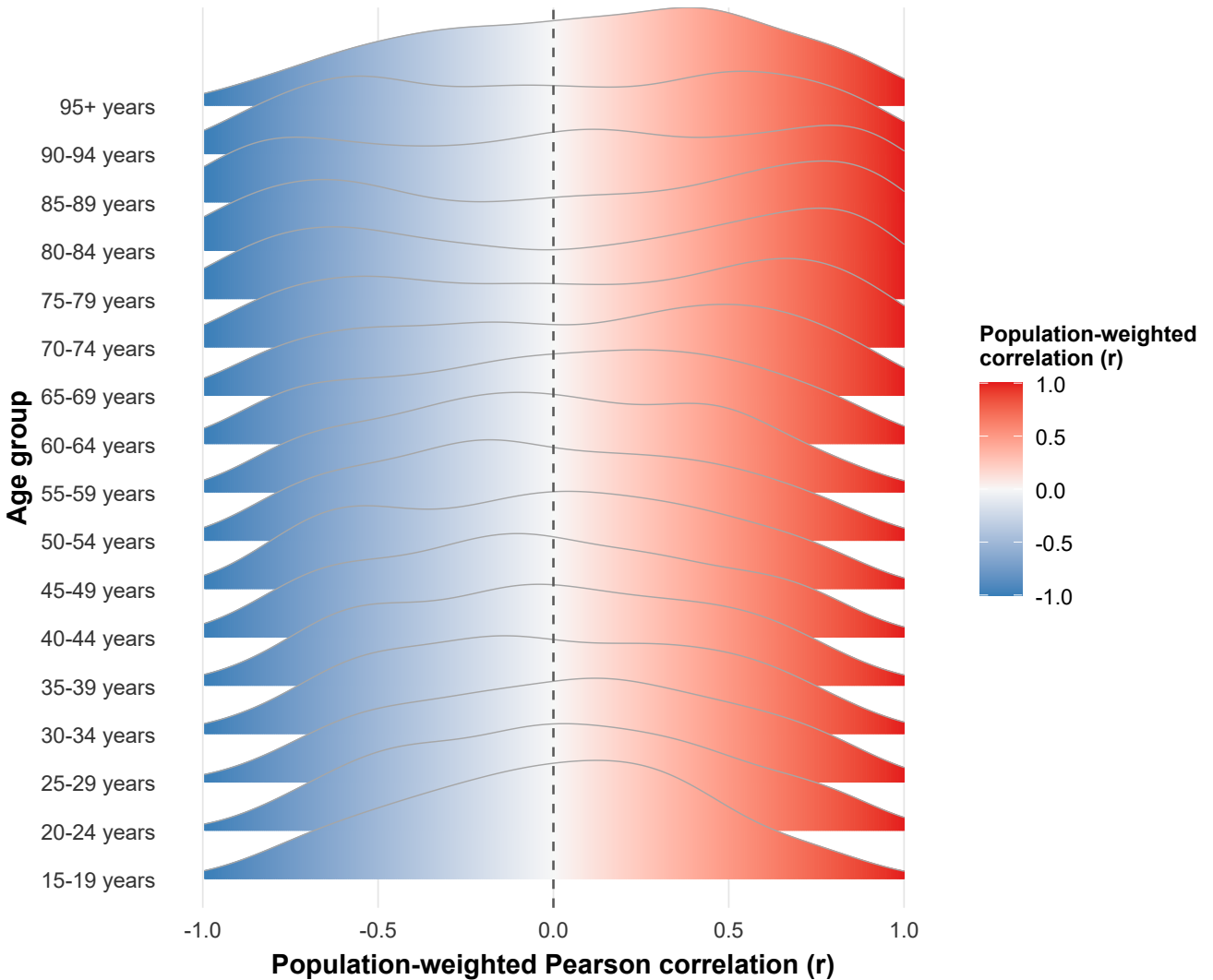
Population-weighted temporal correlation between IHD and DD by country and age group (Male, 1992-2021)
