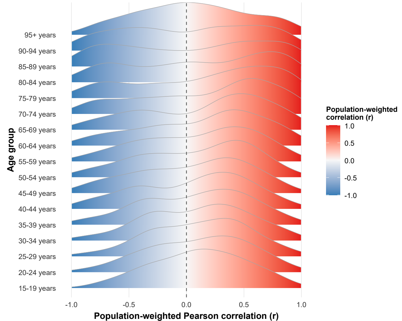
Population-weighted temporal correlation between IHD and DD by country and age group (Female, 1992-2021)
