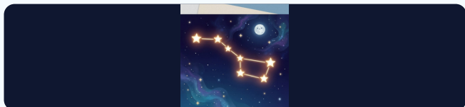
Big Dipper
