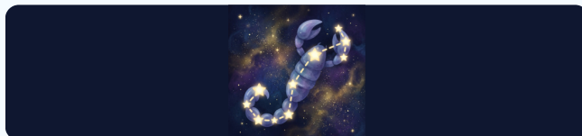
Scorpius
