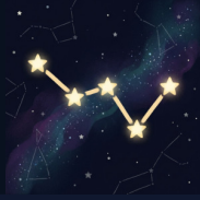
Cassiopeia
