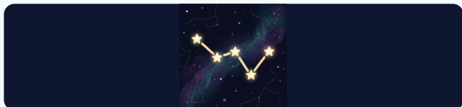
Cassiopeia
