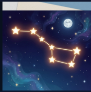
Big Dipper
