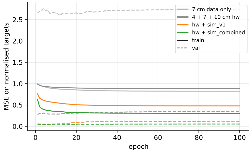
(a) Dynamics-MLP training — linear scale
