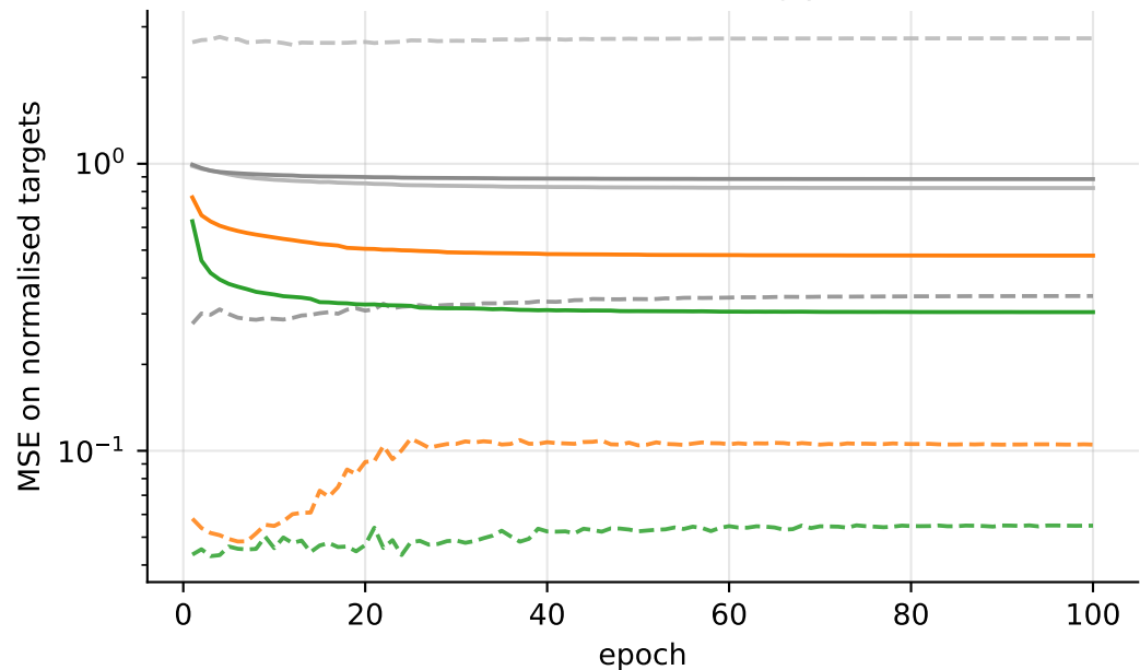
(b) Same curves, log-y
