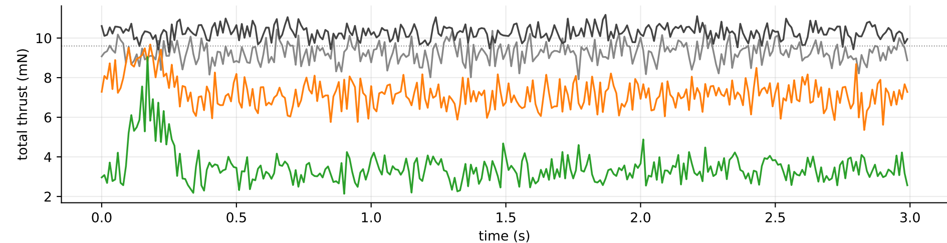
(b) CEM-commanded total thrust
