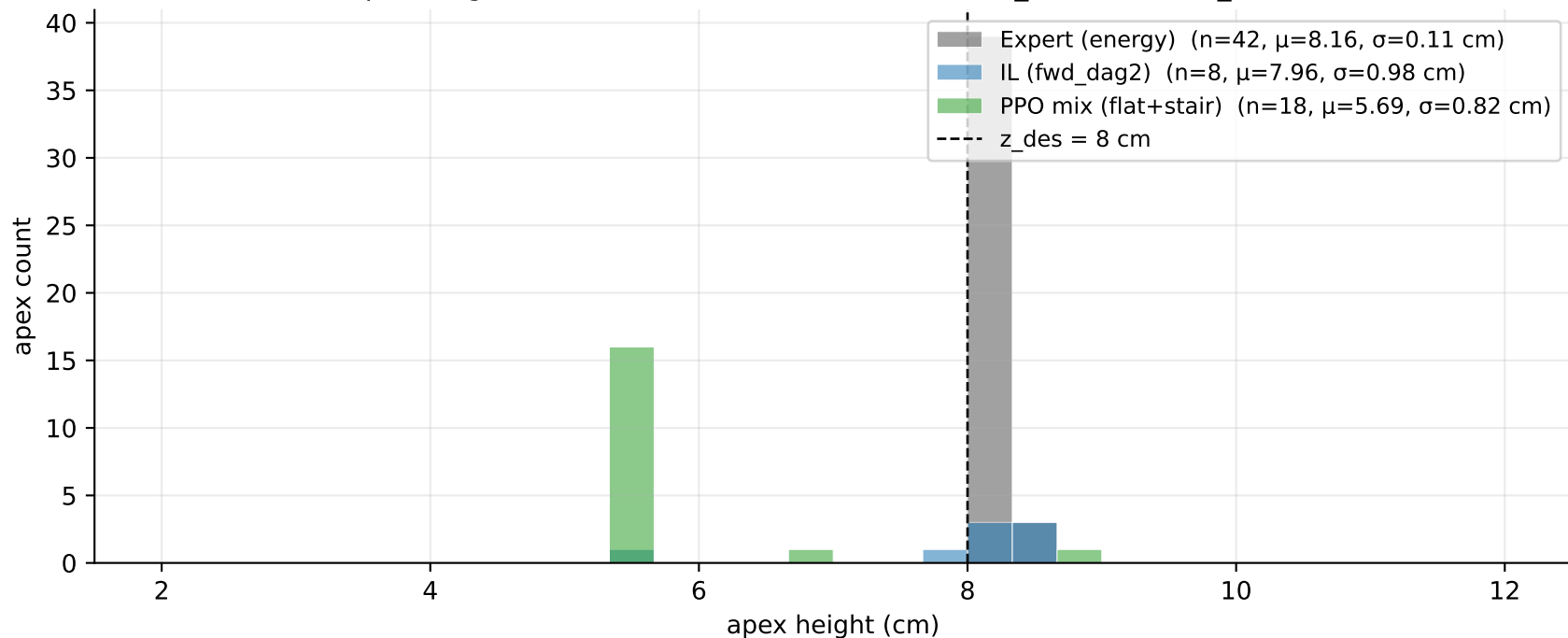
Apex-height distribution — 10 s of flat hover at z_{\text{des}}=8 cm, v_{x_{\text{des}}}=0
