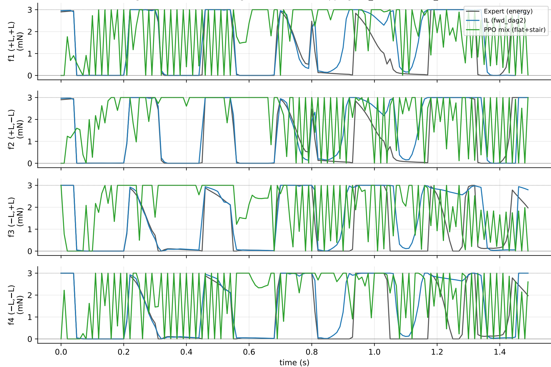
Per-wing force commands during 1.5 s of forward hopping ( v_{x\_des}=3 cm/s, z_{des}=8 cm)
