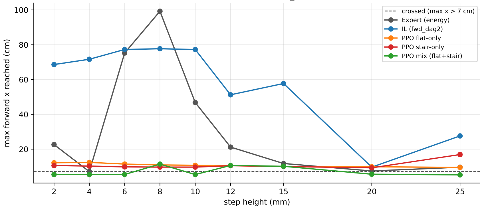
Single-step crossing vs step height ( x_0 = -5 cm, v_{x\_des} = 3 cm/s, step depth = 20 mm)
