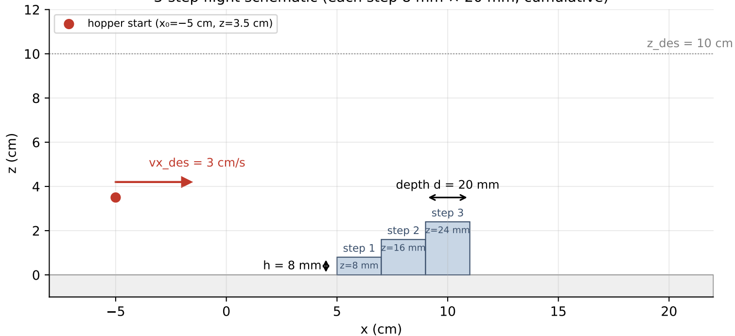
3-step flight schematic (each step 8 mm × 20 mm, cumulative)
